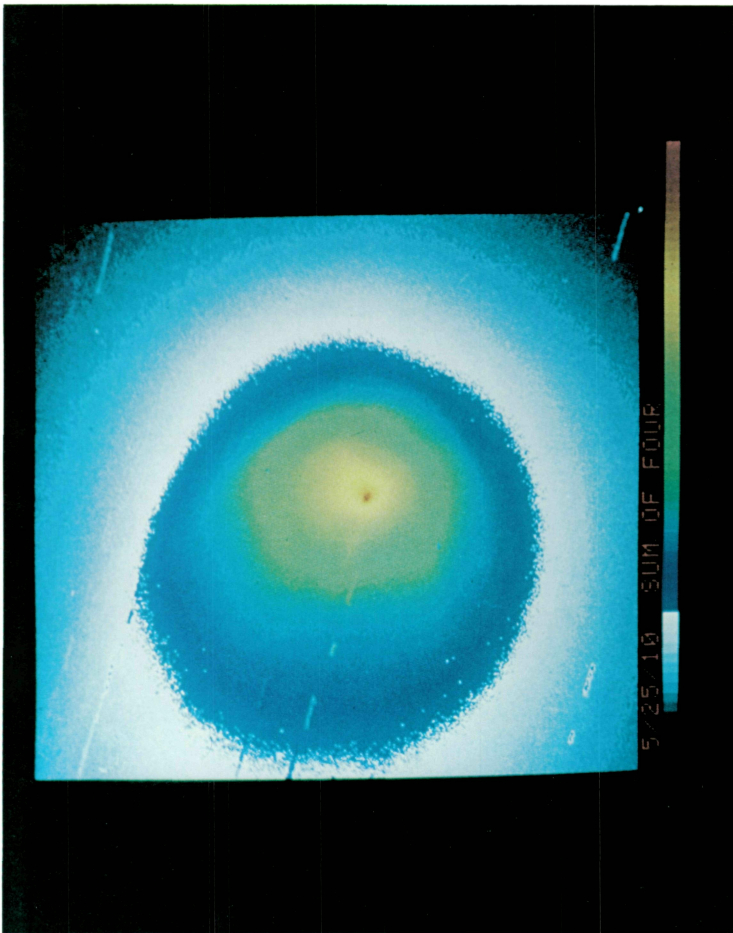
Figure 2. Psuedo-color representation of the sum of the four images of comet Halley obtained on May 25, 1910 at Helwan, Egypt.
